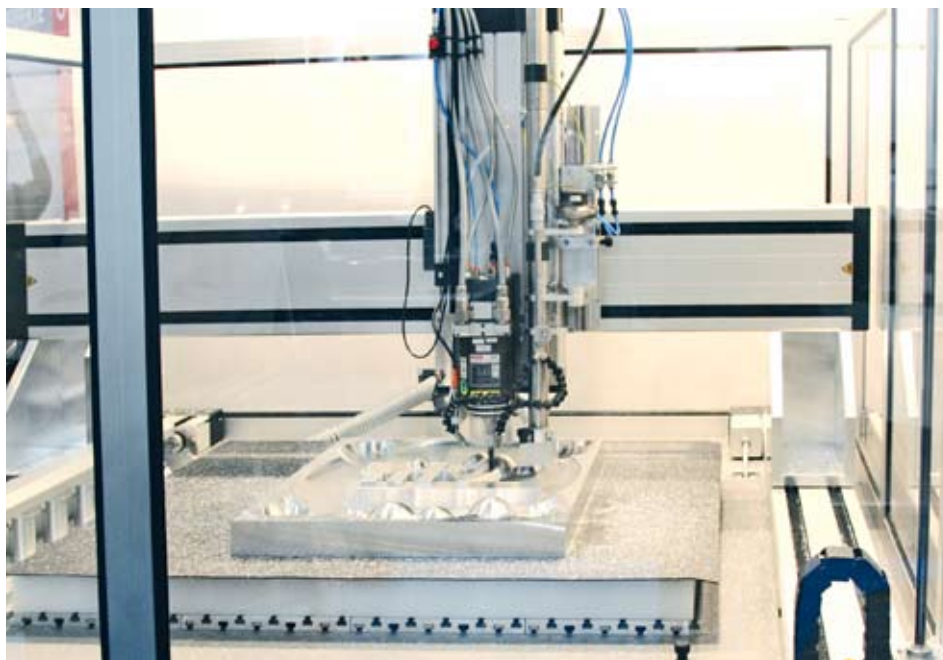
CAM 1010 Premium processing a three-dimensional form out of 50 mm thick aluminium.
